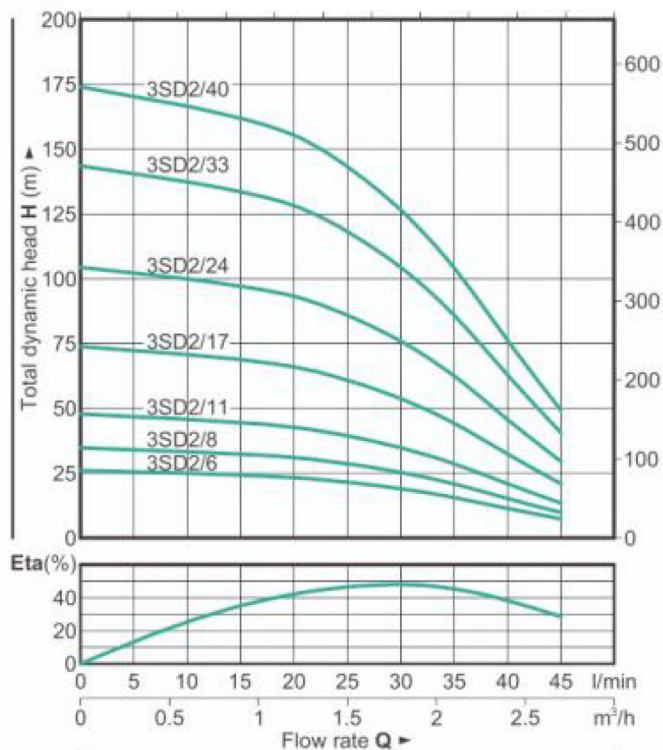
PERFORMANCE DATA 50Hz
